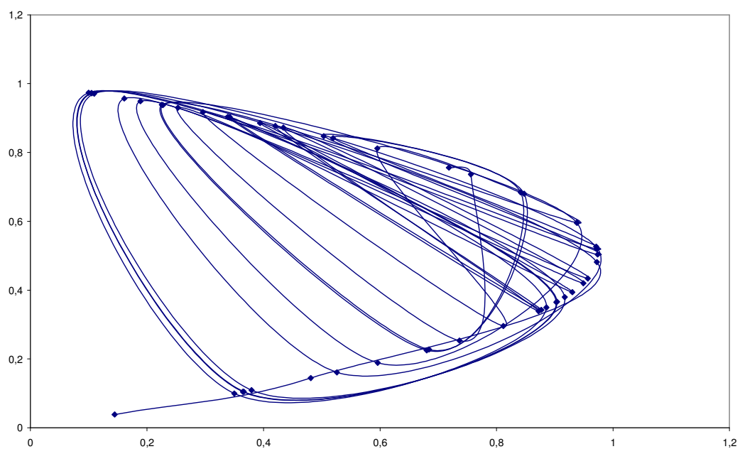
Graph 6: Strange attractor
