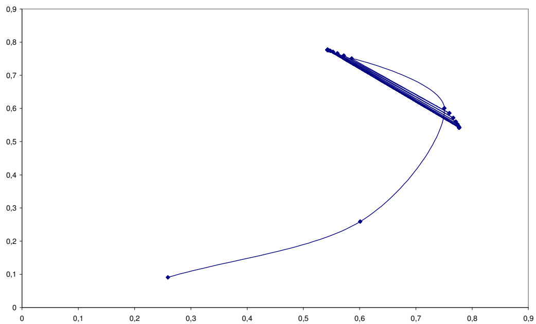
Graph 5: Periodical attractor
